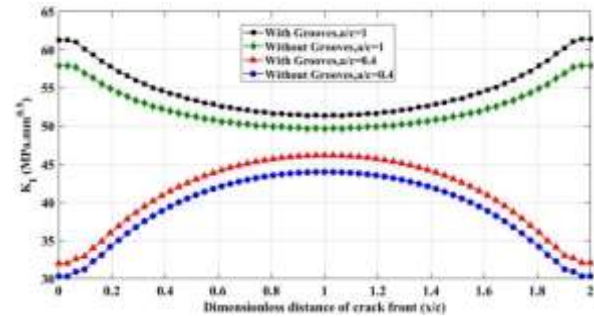
Fig. 20 Diagram of changes in the SIF k_I in the circumferential crack front for a titanium rotating disk at 9000 rpm in the grooved and ungrooved condition
